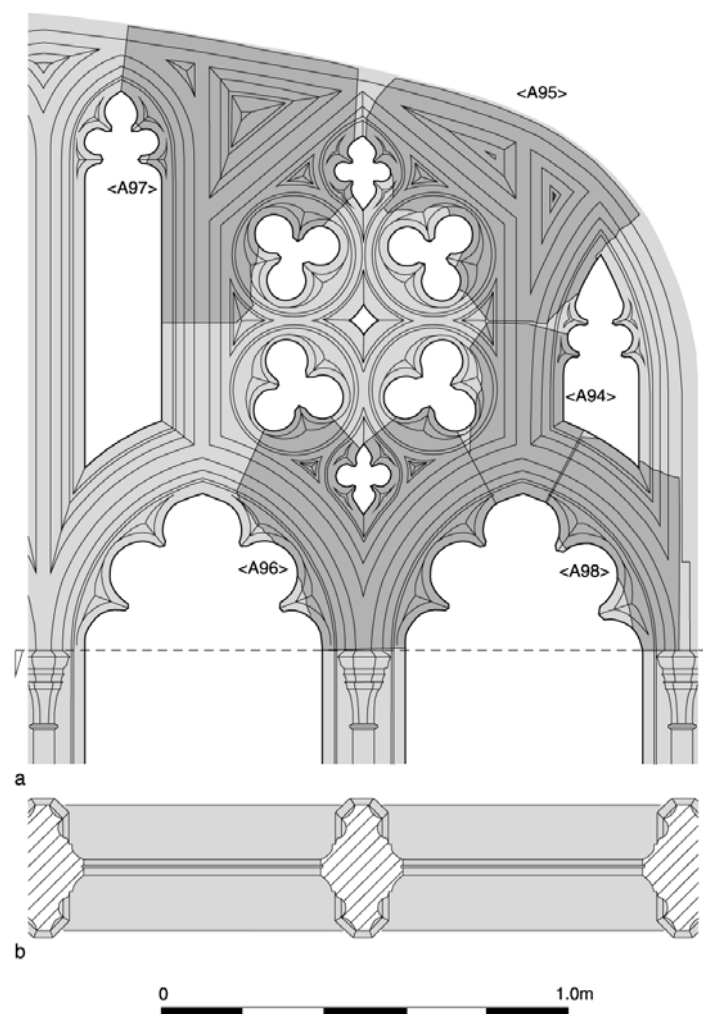
Fig 3 Reconstruction of half of a bay of tracery in a cloister arcade of the late 14th century at Merton Priory in south-west London. Although there have been archaeological excavations on the priory site, these pieces came from another excavation on the site of Henry VIII's Nonsuch Palace a short distance away. Though pieces from parish churches and chapels may be simpler, the principles of measurement and reconstruction from these fragments are the same. Drawing by Mark Samuel, based on the work of Terry Ball (see also Miller and Saxby 2007)
